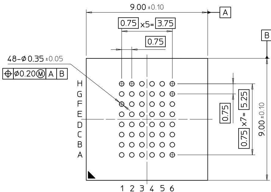
BOTTOM VIEW
