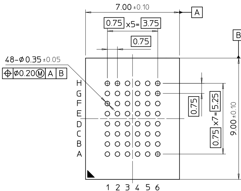
BOTTOM VIEW
